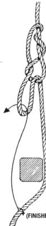
ROSENDAHL OR ZEPPELIN KNOT
